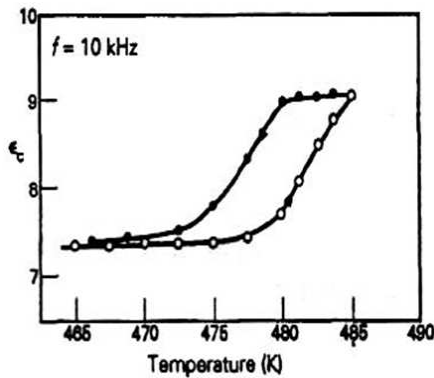
Fig 4. Dielectric constant vs temperature
