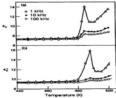
Fig 3. Dielectric constant of EDS as a function of temperature
