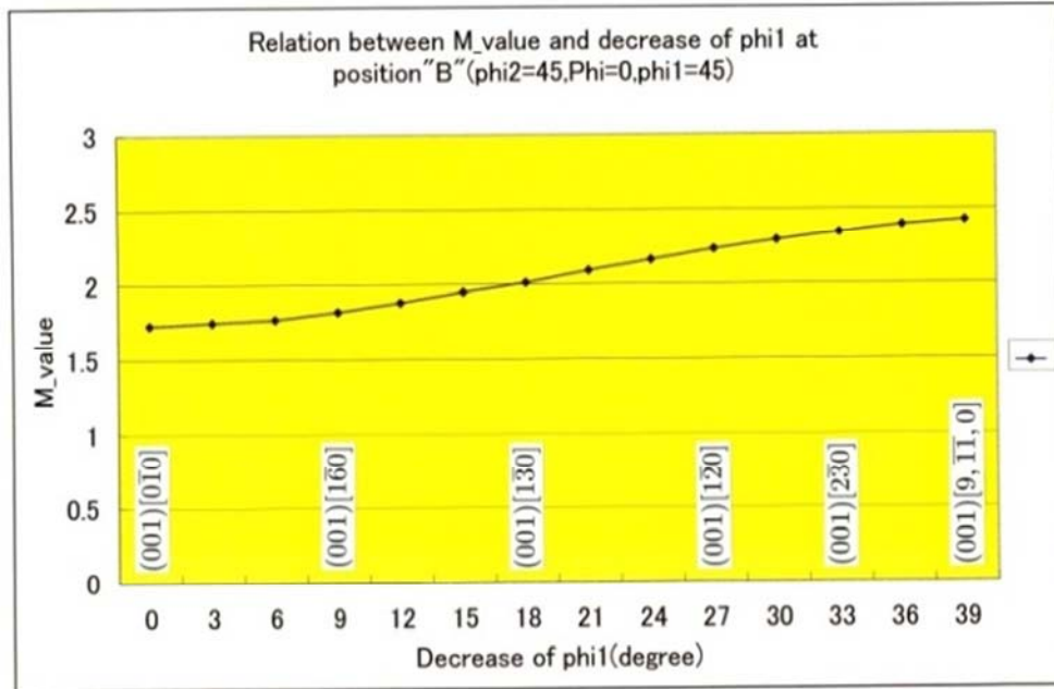
Figure 8. Change of Taylor factor M value with decrease of \phi_1 from cube structure \{100\}\langle 001\rangle at point B in the ODF coordinates of Figure 5(1) of fcc metal under cold rolling.
