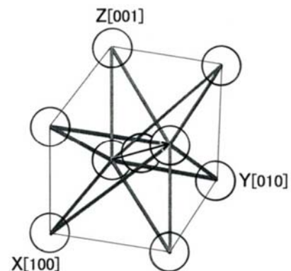
Figure 2. Three kinds of {110} planes composed of {110}, {101} and {011} ones around the principal Z [001] axis with a common slip direction <111> in bcc crystal.
