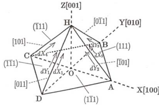
Figure 1. Illustration of the {111}<110> glide systems in the Z ([001]) group and the principal axes for fcc metal in the present model.
