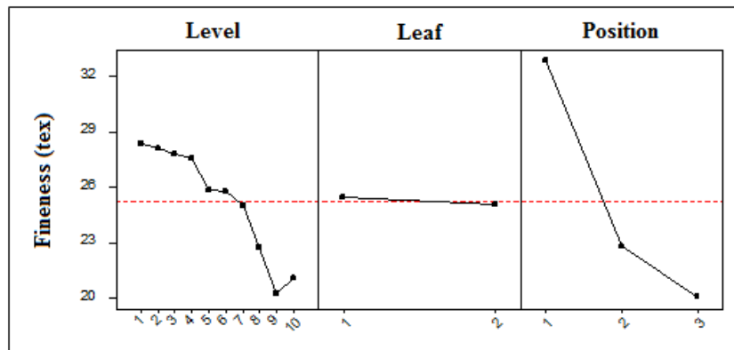
Figure 9. Main effects plot for the fineness.
